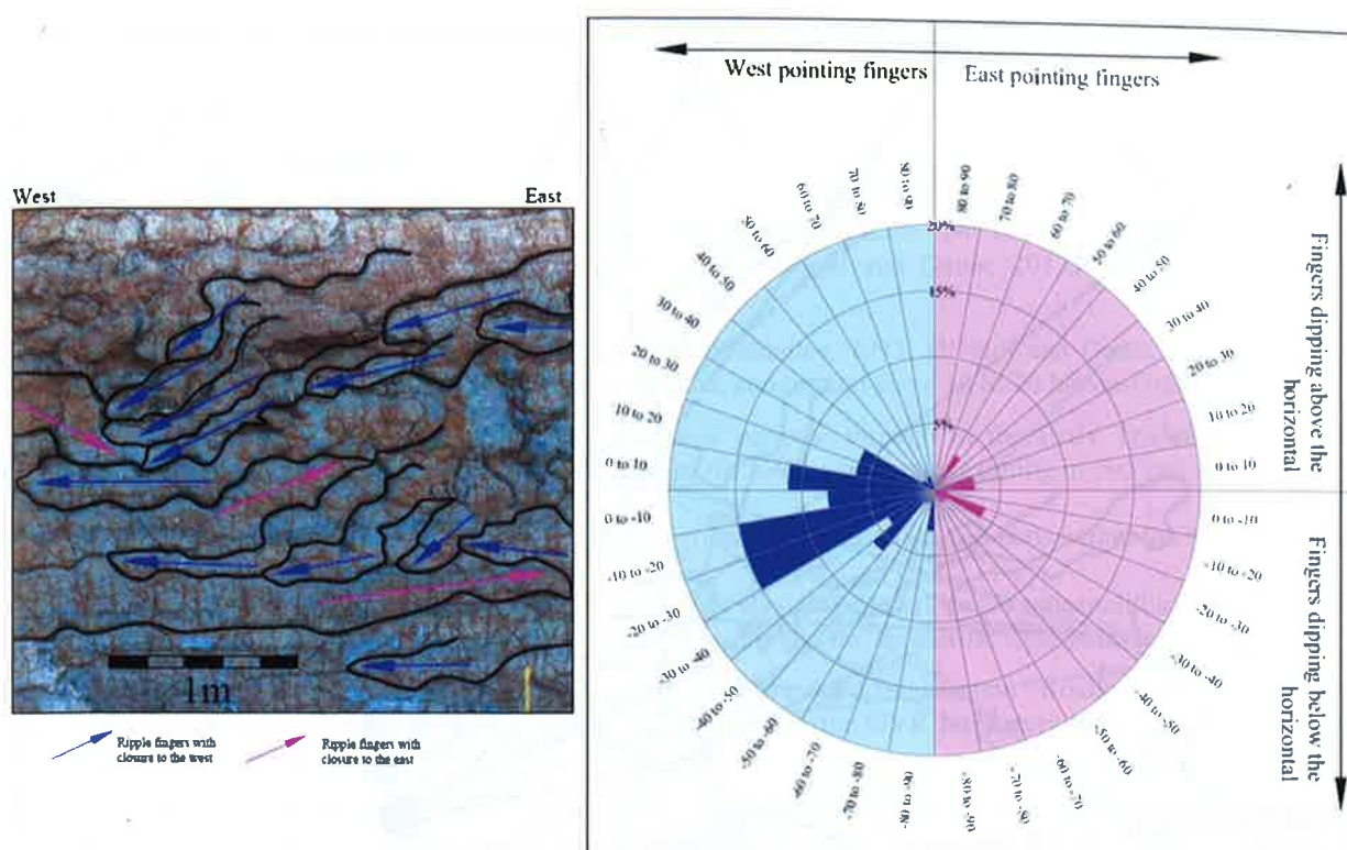
Figure 6: Surface ripple orientation assessment (left). Graphical summary of ripple closure orientations (right).
