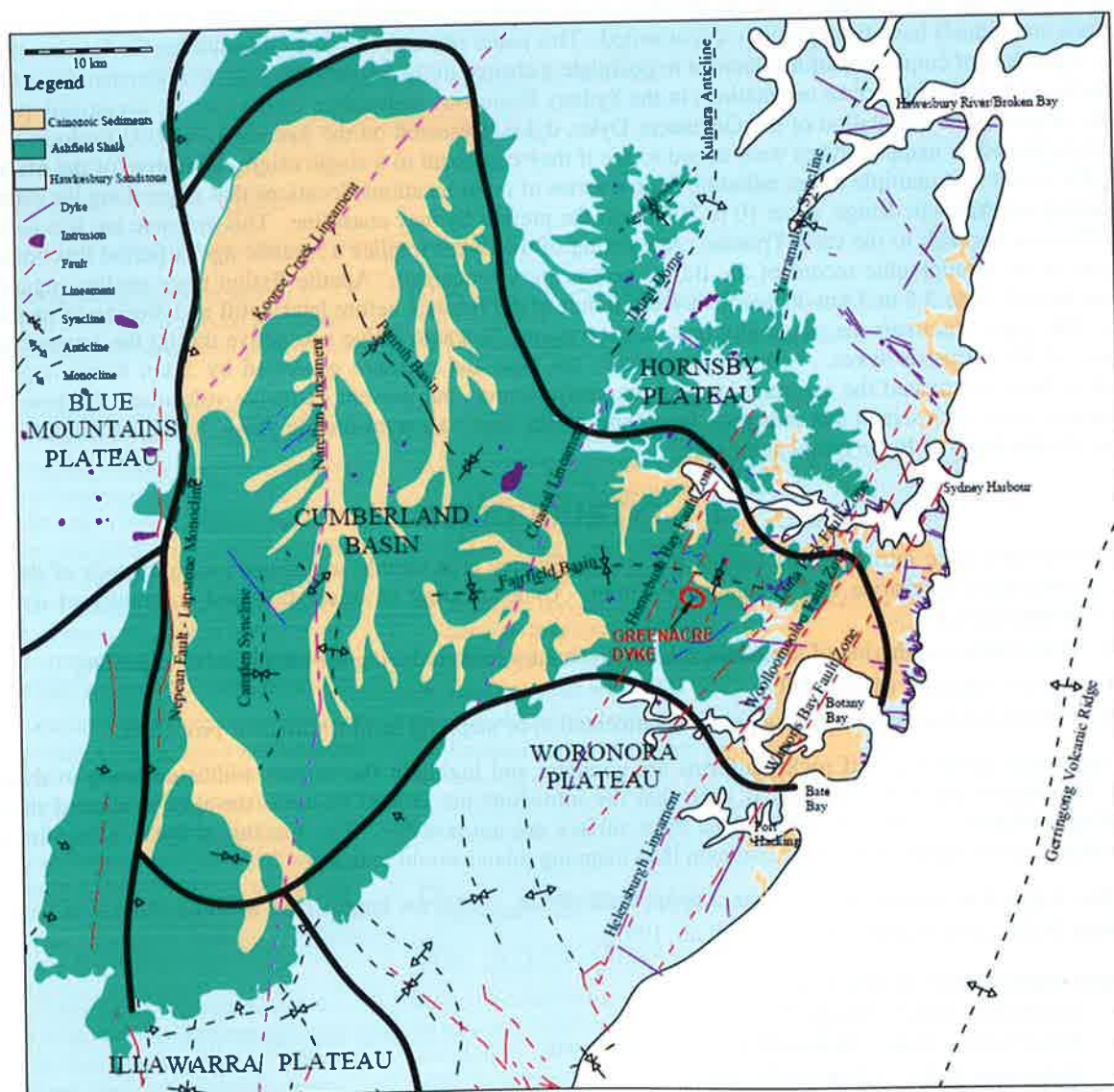
Figure 1: Structural components of the Sydney Basin after Herbert (1983); Bradley (1993); Och et al. (2009); Branagan (2000); unpublished mapping known to and by author.
